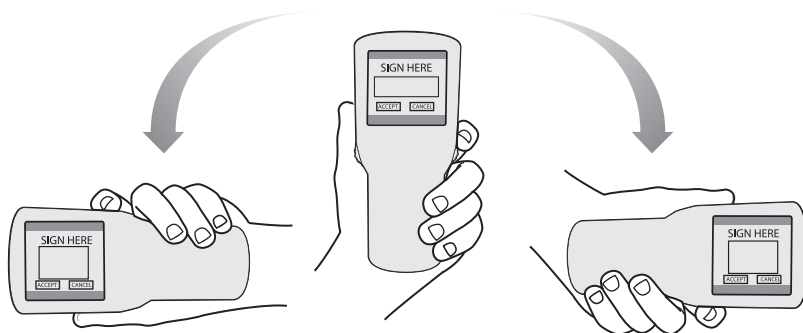
Figure 84: Display Orientation
