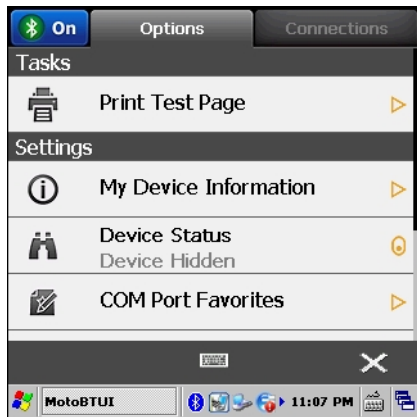
Figure 94: MotoBTUI Window
