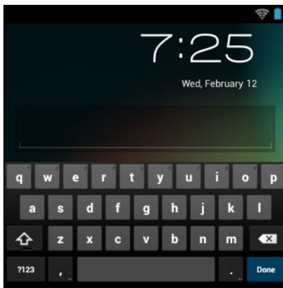
Figure 57: Password Screen
